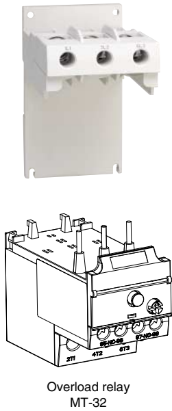
Separate mounting adapter
