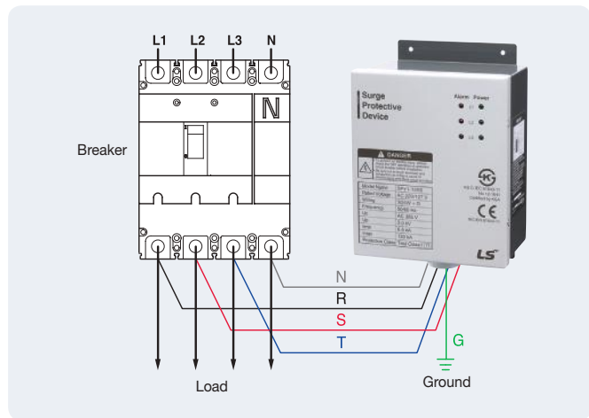
Three phase 4W+G (SPY Series)
