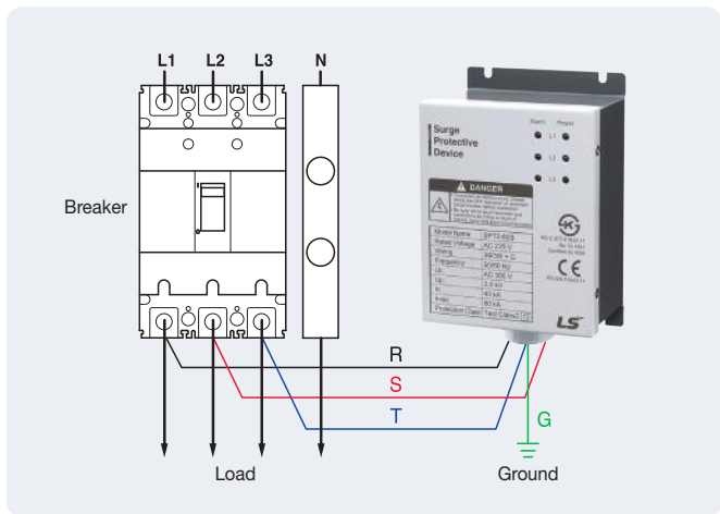
Three phase 3W+G (SPT Series)
