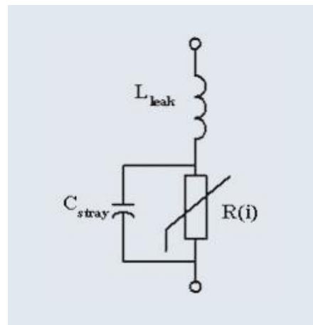
MOV equivalent circuit
