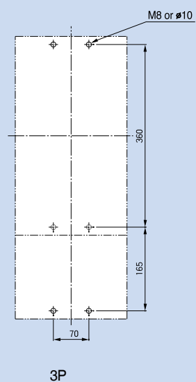
Panel drilling
