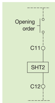
Wiring diagram
